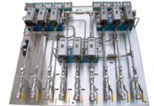
9 Line Priority Fill Panel
